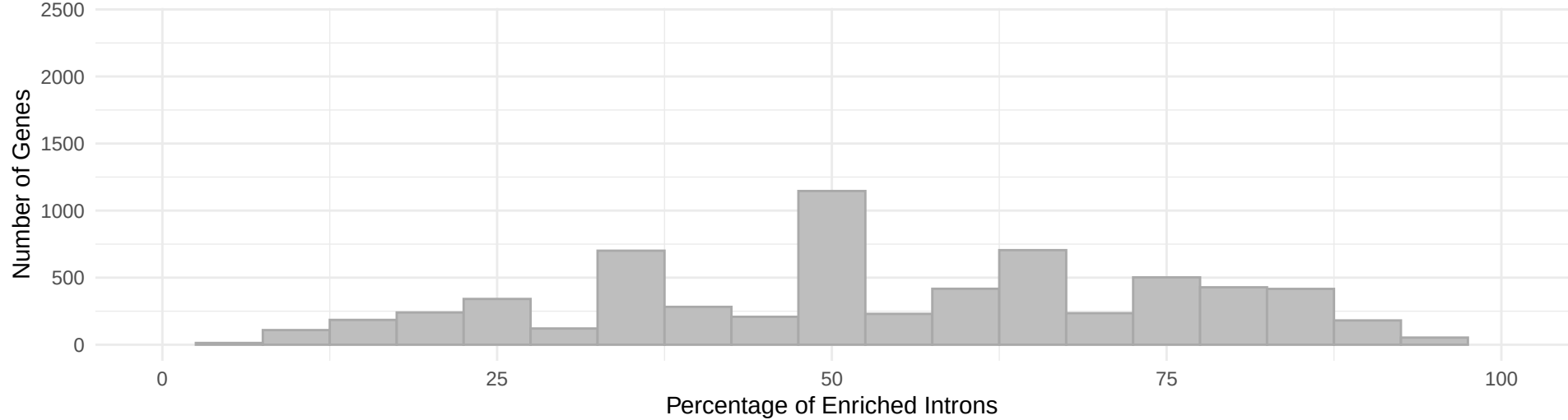
GSK591_Chromatin Percentage of Enriched Introns per Gene
